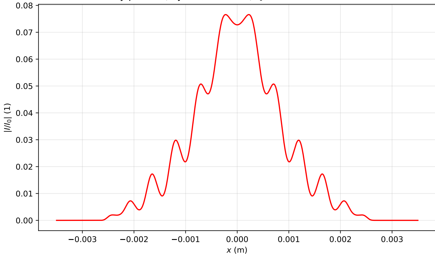
Intensity profile I(x, y = 0, z = 3.025)/I_0 , P_{in}=2.0P_{cr} , artificial time
